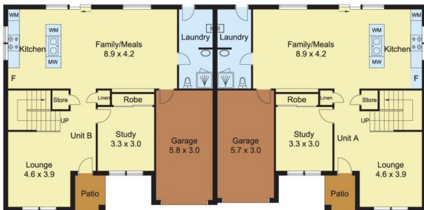
GROUND FLOOR
