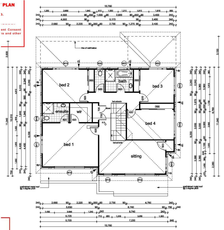
First Floor 1:100
