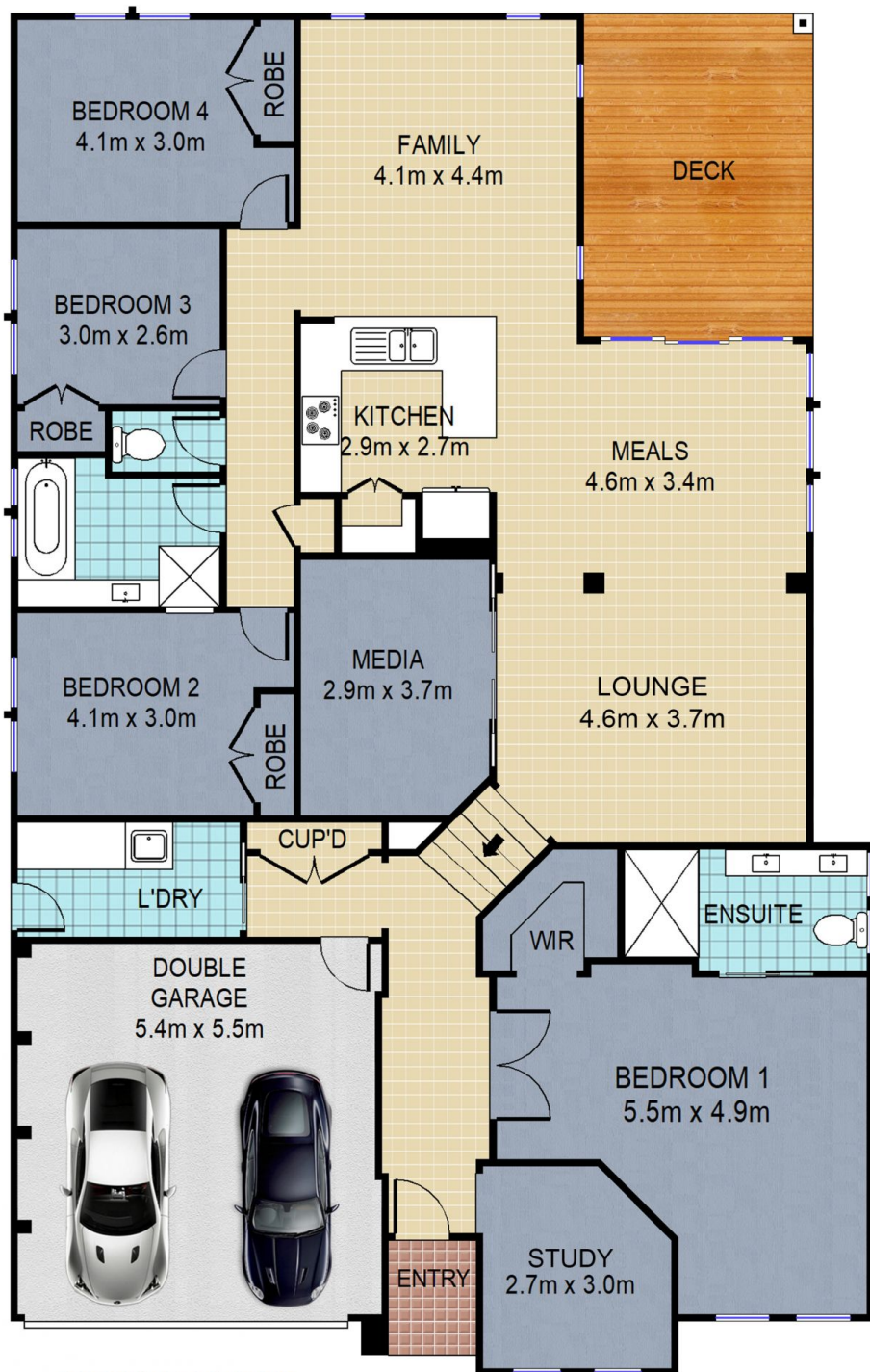
GROUND FLOOR
