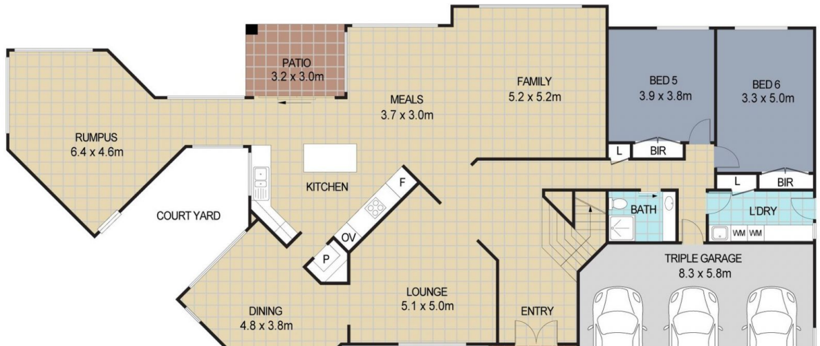
FIRST FLOOR
